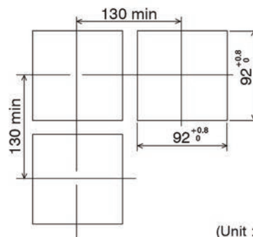
Panel Cutout
