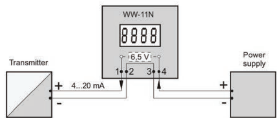
Electrical diagram
