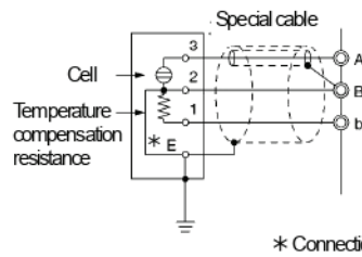
Electric conductivity recorder 3-cored input
