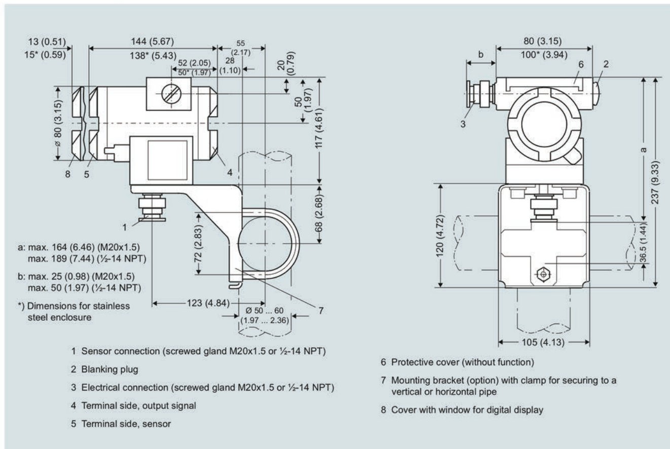
SITRANS TF, dimensions in mm (inches)
