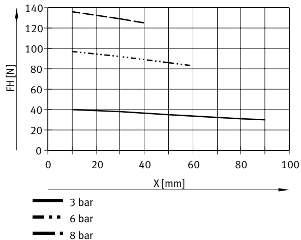
Gripping force F per gripper jaw as a function of operating pressure and lever arm x – Internal gripping (opening), double-acting – DHPL-16-80-...-A
