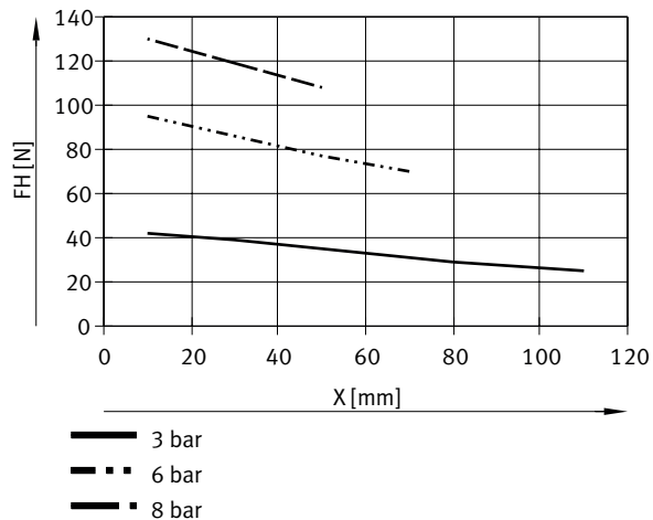
Gripping force F per gripper jaw as a function of operating pressure and lever arm x – Internal gripping (opening), double-acting – DHPL-16-30-...-A
