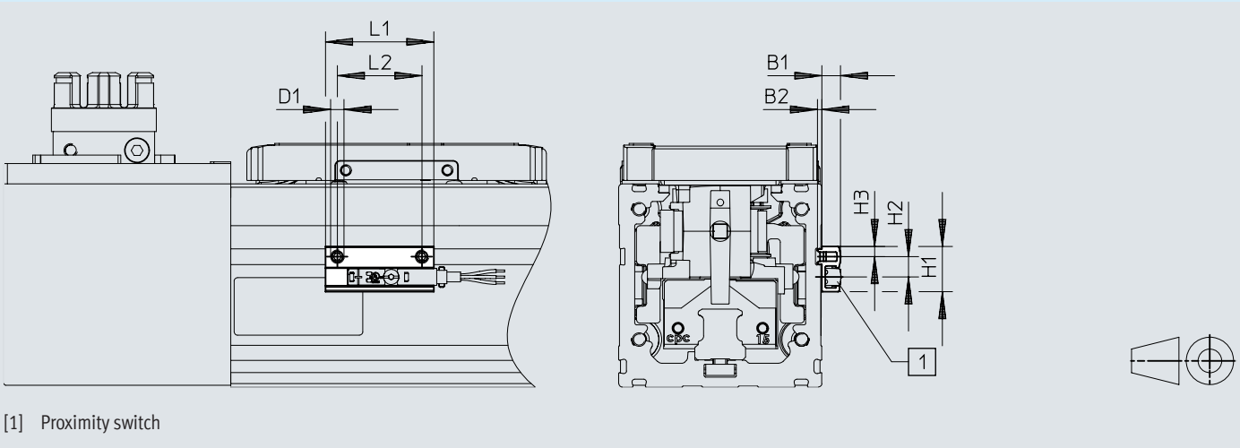
Dimensions – Sensor bracket EAPM-L2-SH
