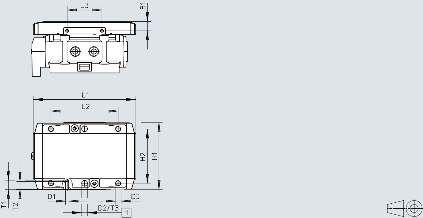
Dimensions – Toothed belt axes ELGC-TB-KF, size 60 (slide)
