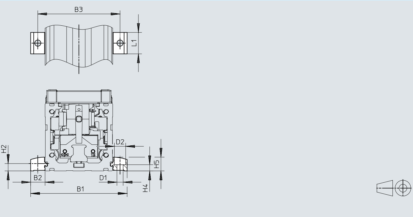
Dimensions – Profile mounting EAHF-L2-...-P-S
